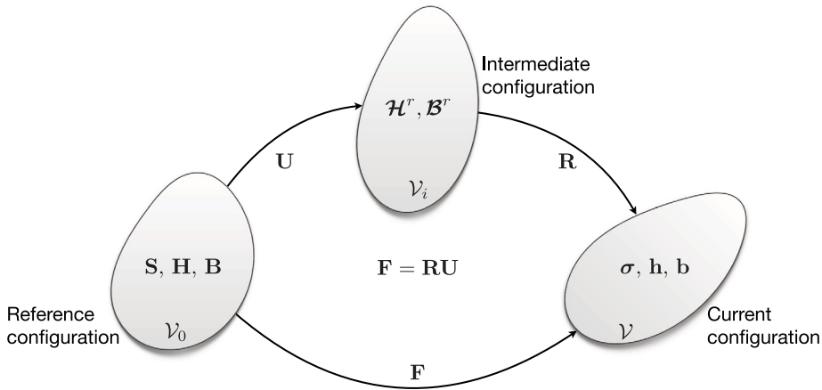
Fig. 1. Definition of the reference, intermediate and current configurations of volume \mathcal{V}_0 , \mathcal{V}_i and \mathcal{V} , respectively, along with the different field variables defined therein.
